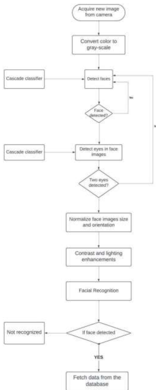
Figure 1.3 Flow diagram of the Proposed System
